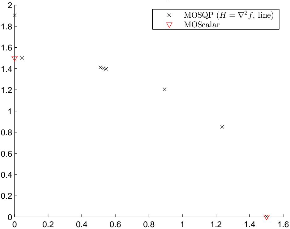
DTLZ5n2_adapted
